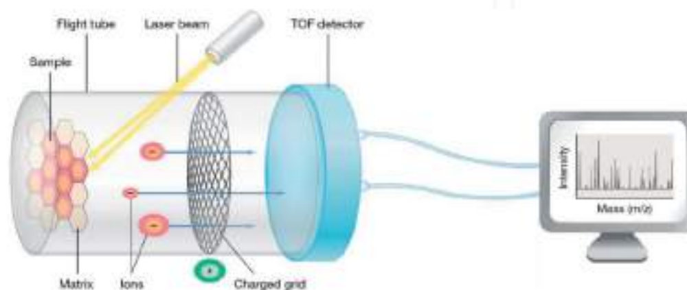
Figure 11. MALDI-TOF mass spectrometry device [11].
