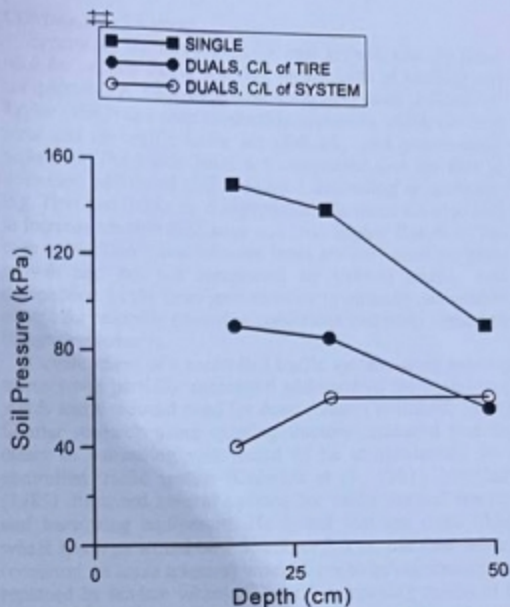
Figure 10. Soil pressures measured beneath single and dual tires (Taylor et al., 1986).
