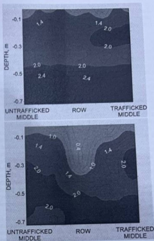
Figure 7. On top is cone index profile (MPa) showing soil that is compacted beneath row. On bottom is cone index profile showing benefit of subsoiling operation beneath row (Raper et al., 1998).
