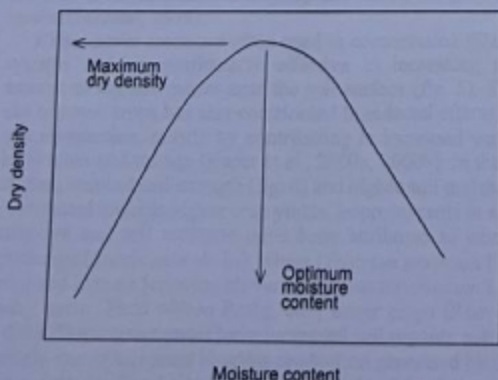
Figure 4. Schematic compaction curve, showing the maximum compaction at the optimum moisture content.
