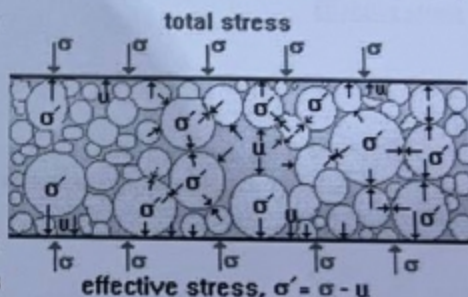
Effective stress
